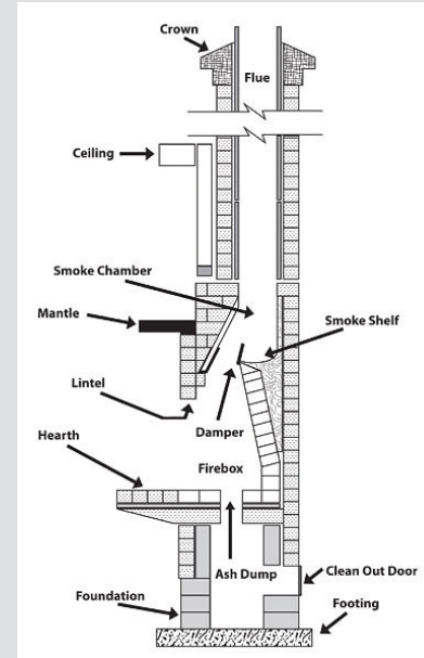
M Masonry fireplace
