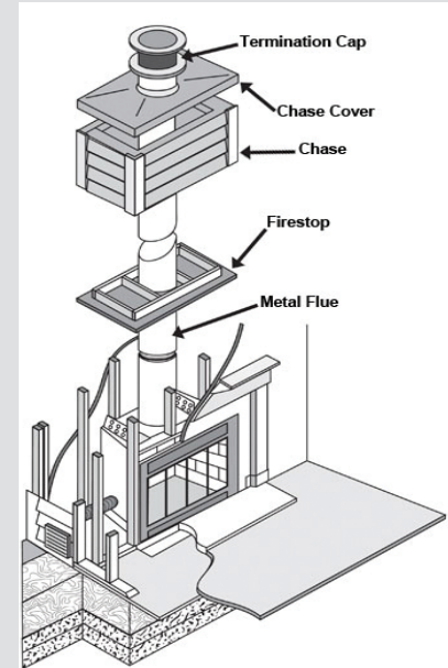
ZC Zero Clearance fireplace
